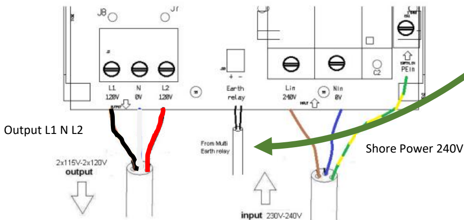
Wiring diagram: MTR-100
